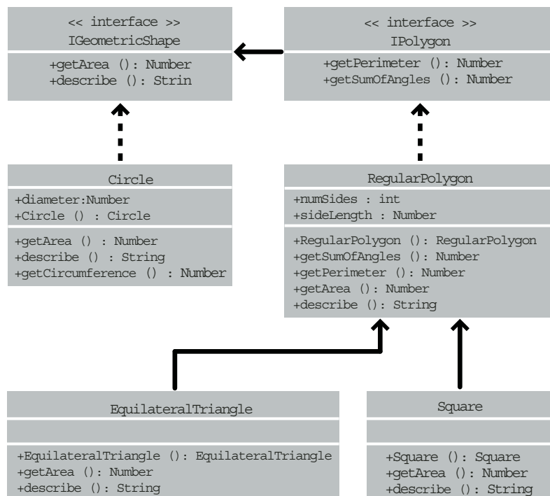
GeometricShapes 示例类
